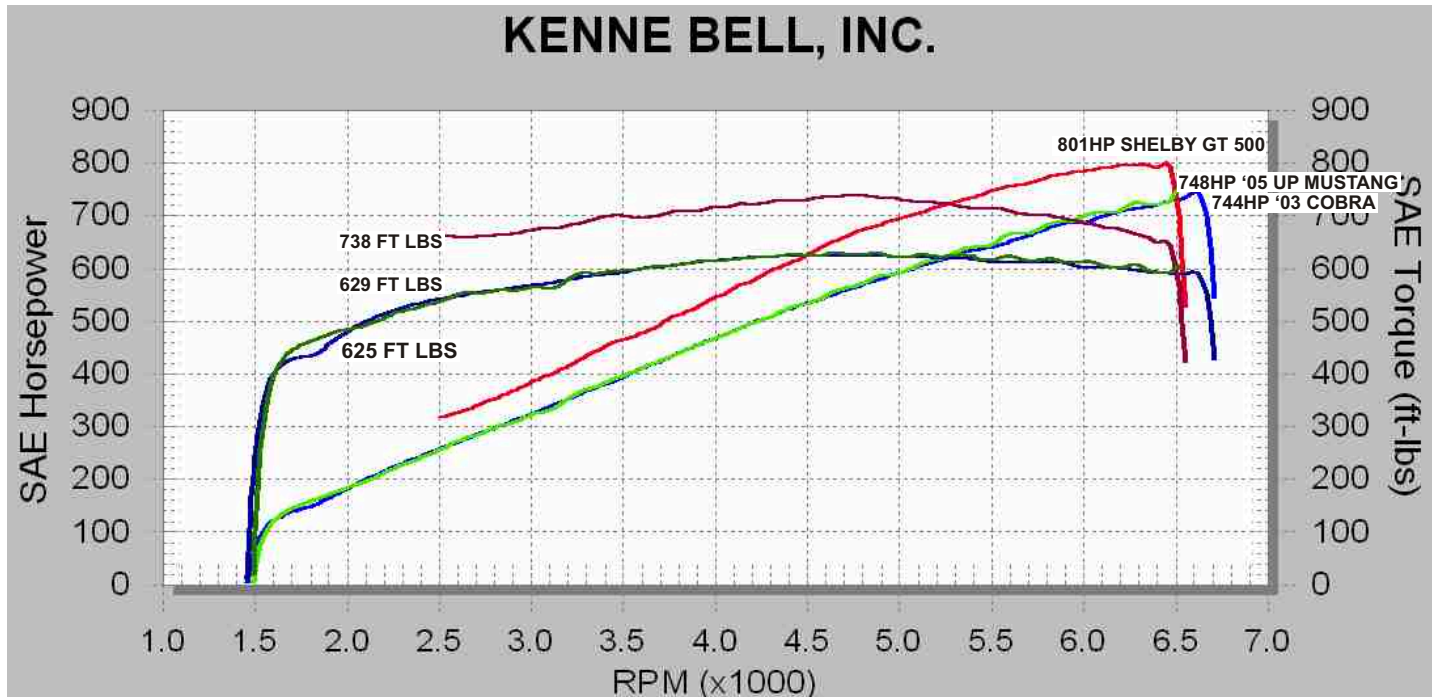
MAMMOTH™ 2.8H KITS - 23 PSI SHELBY GT 500, '05 UP MUSTANG, '03-'04 COBRA 100% STOCK ENGINE W/CAT BACK REAR WHEEL HP & TORQUE
